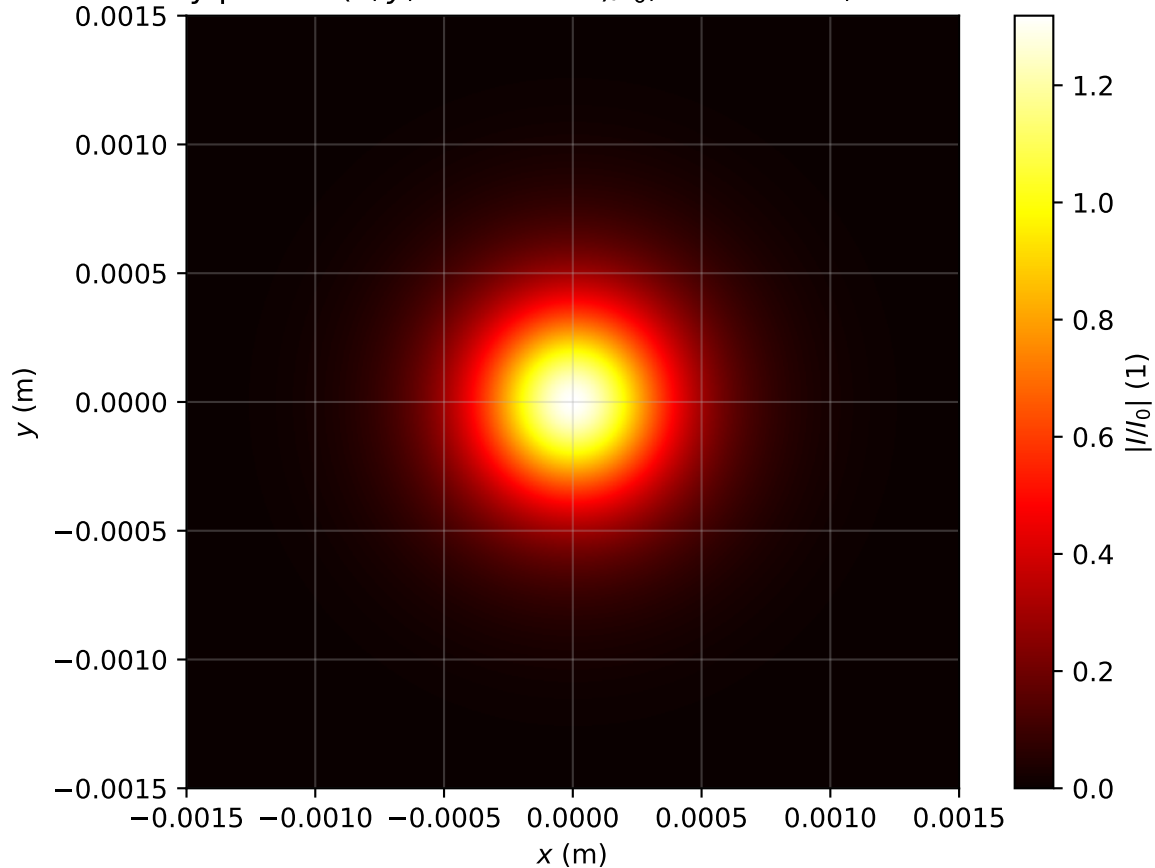
Intensity profile I(x, y, z = 1.115m)/I_0 , Pin=0.8Pcr, artificial time
